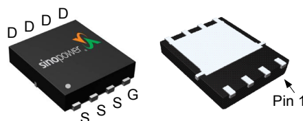
DFN5x6-8
