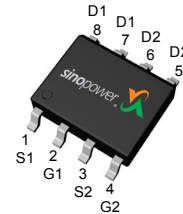
Top View of SOP-8
