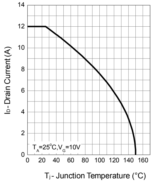
Drain Current
