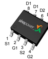
Top View of SOP-8
