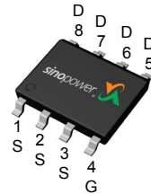
Top View of SOP-8
