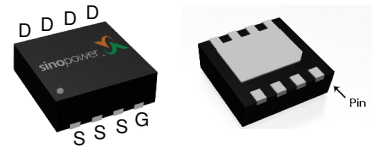
DFN3.3x3.3-8(Saw-EP)
