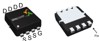
DFN3x3A-8_EP
