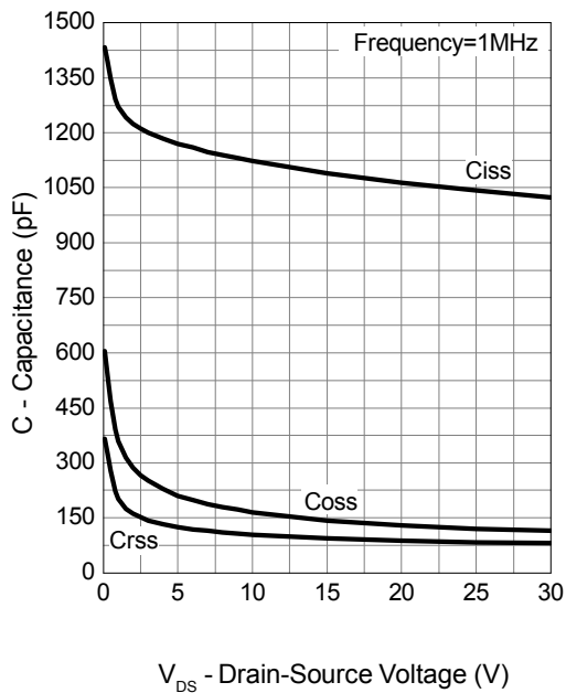
Capacitance
