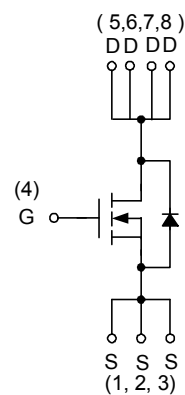
N-Channel MOSFET
