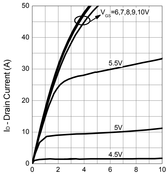
Output Characteristics
