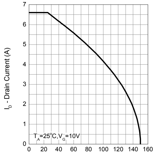
Drain Current
