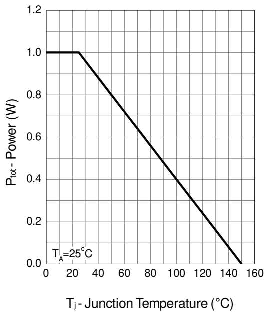
Power Dissipation
