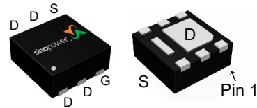
DFN2x2A-6_EP
