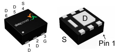
DFN2x2A-6_EP
