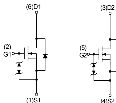
N-Channel MOSFET
