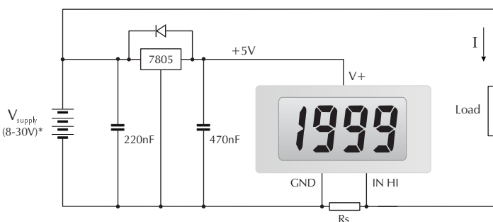
Measuring current.
