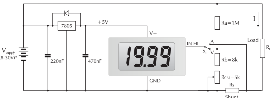
Measuring supply voltage and current.
