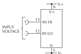
Check Links 1, 2, 3 & 4 are SHORTED Measuring a floating voltage source of 200mV full scale.
