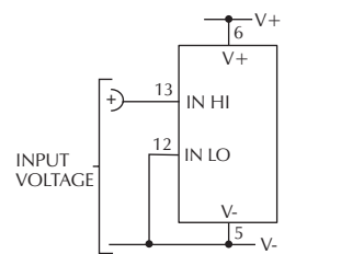
Check Links 1, 3 & 4 are SHORTED. Measuring a single ended input referenced to supply (DPM 160S).
