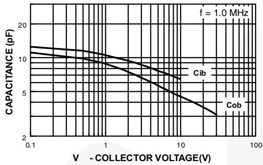
Figure 7. Input and Output Capacitance vs. Collector Voltage
