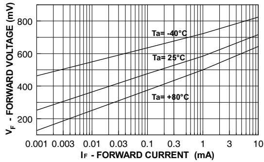
Figure 7. Forward Voltage vs. Ambient Temperature V_F - 1.0 \mu\text{A} - 10 mA (- 40 to +80^\circ\text{C} )
