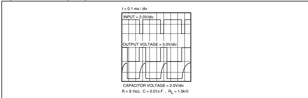
Figure 5. Timing diagram
