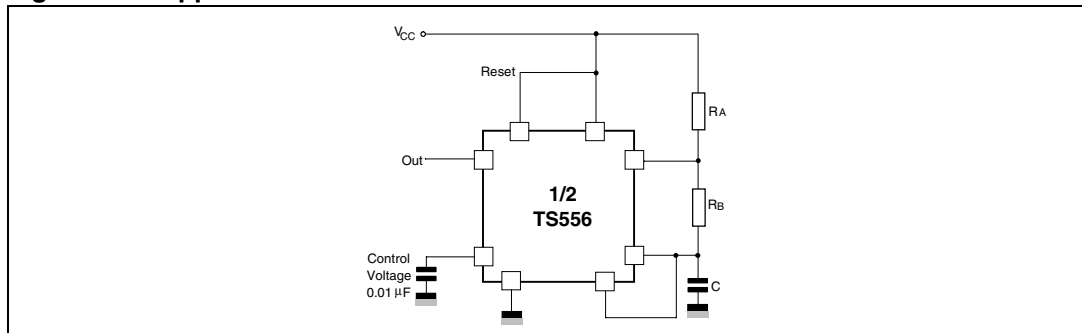
Figure 6. Application schematic
