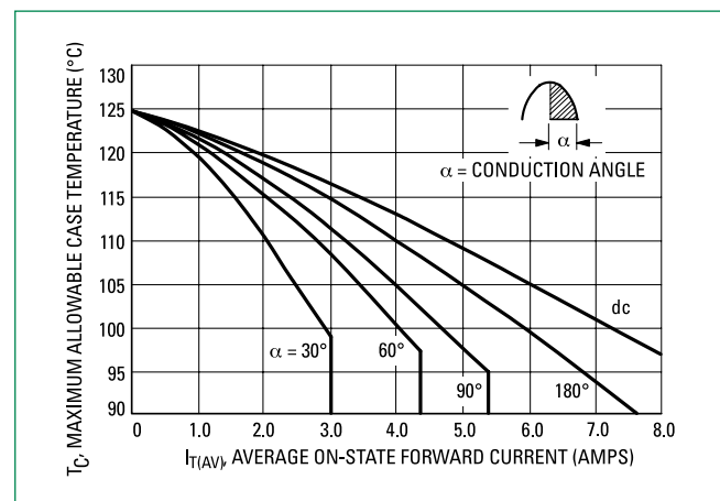
Figure 1. Current Derating
