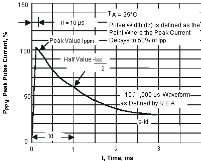
Fig. 3-Pulse Waveform
