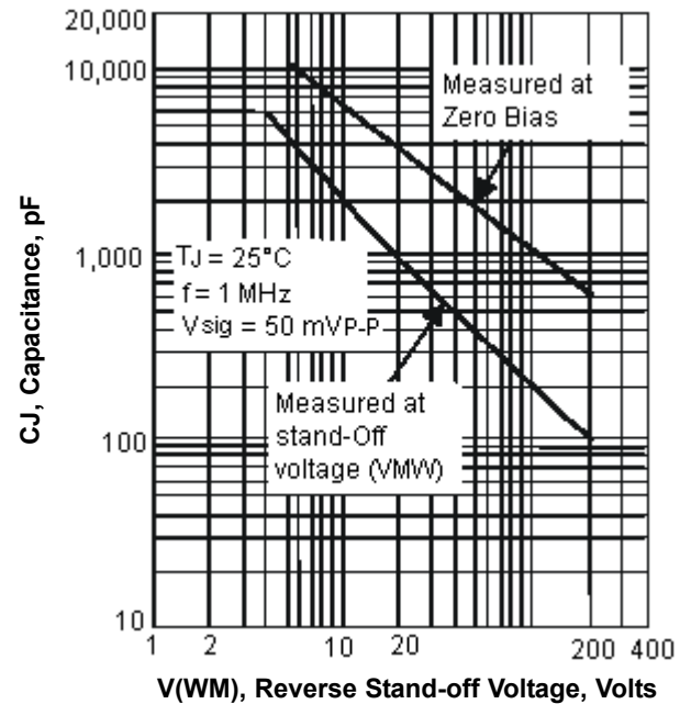
Fig. 4-Typical Junction Capacitance
