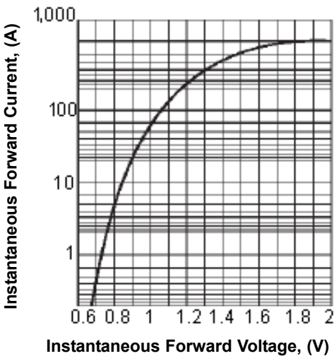
Figure 2 Typical Instantaneous Forward Characteristics at T_J = 25^{\circ}\text{C}
