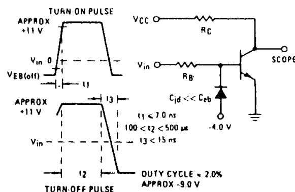
Switching Time Equivalent Circuit
