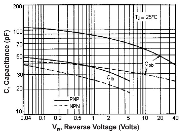
Figure - 4 Capacitances
