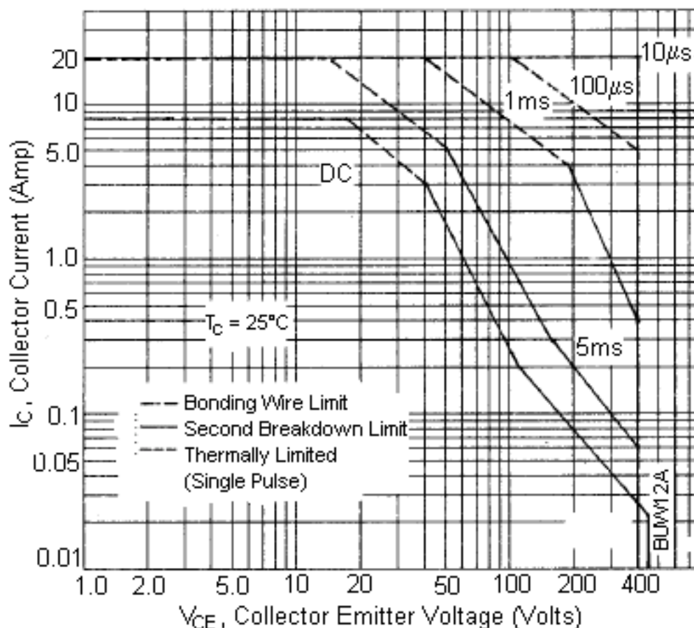
Active-Region Safe Operating Area (SOA)
