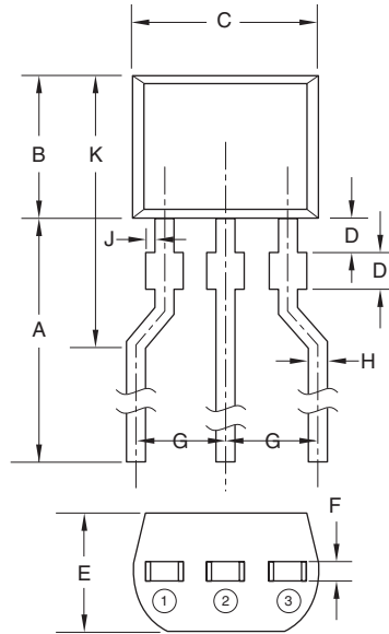
CONNECTION DIAGRAM
