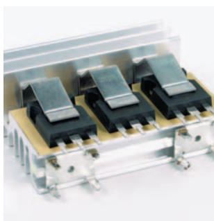
Choose a Sil-Pad that optimizes thermal performance for your mounting method — screw, clip, spring, bar, etc.
