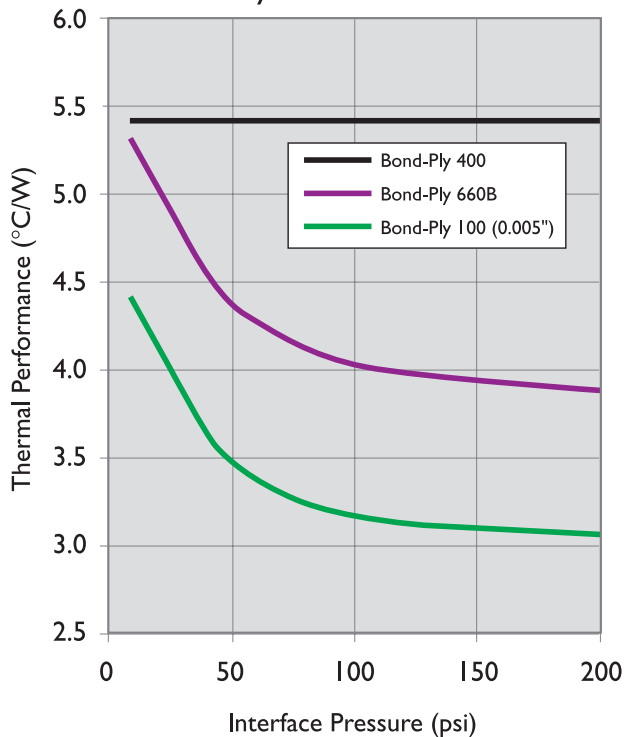
Bond-Ply Thermal Performance
