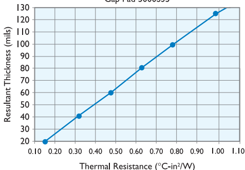
Thickness vs. Thermal Resistance Gap Pad 5000S35
