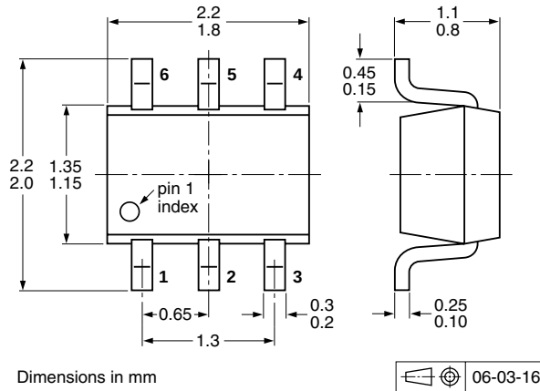
Fig 5. Package outline SOT363 (SC-88)
