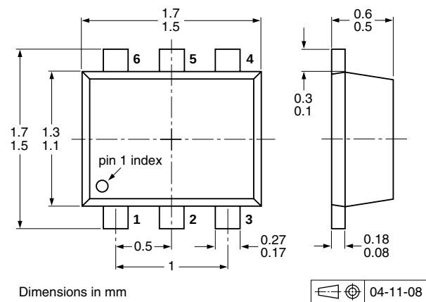
Fig 6. Package outline SOT666
