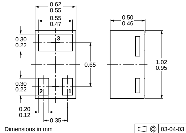
Fig 13. Package outline PDTC143ZM (SOT883/SC-101)
