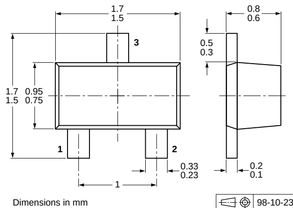
Fig 6. Package outline SOT490 (SC-89)
