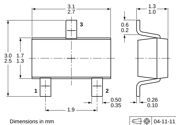
Fig 7. Package outline SOT346 (SC-59A/TO-236)
