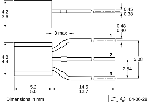
Fig 10. Package outline SOT54A
