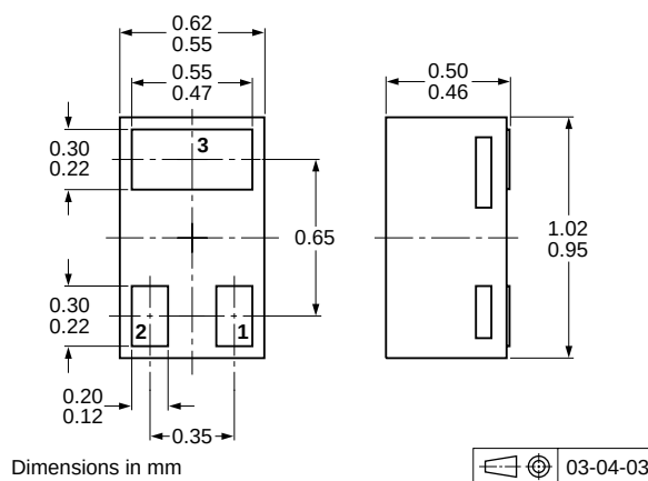
Fig 8. Package outline SOT883 (SC-101)
