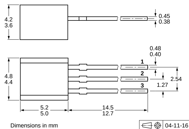
Fig 9. Package outline SOT54 (SC-43A/TO-92)
