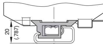
9102100000 TS32 adapter
