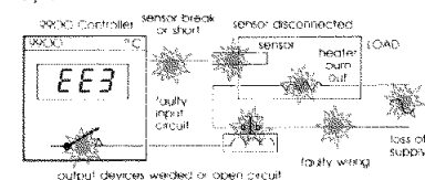
Fig. 3 Typical faults detected by LBA
