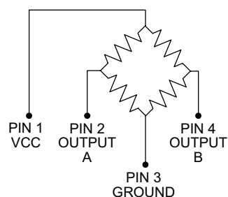
Figure 1. Circuit Diagram
