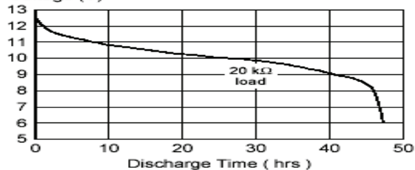
Normal Rate Discharge Voltage (V)
