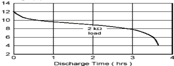
High Rate Discharge Voltage (V)
