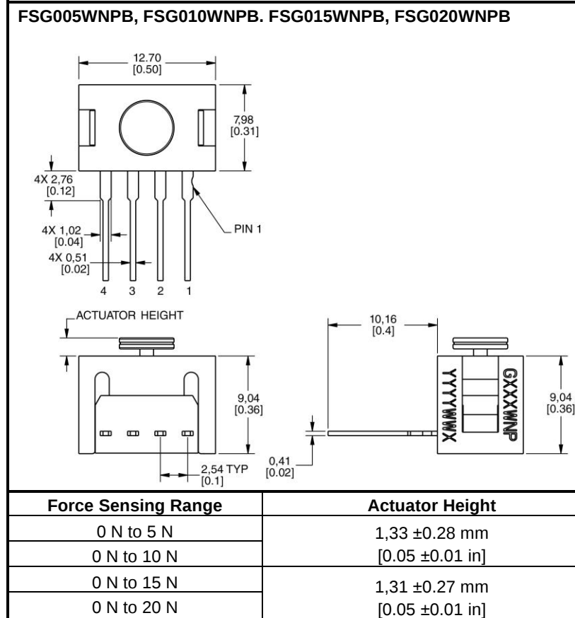
Figure 2. Sensor Mounting Dimensions (For reference only: mm/[in].)
