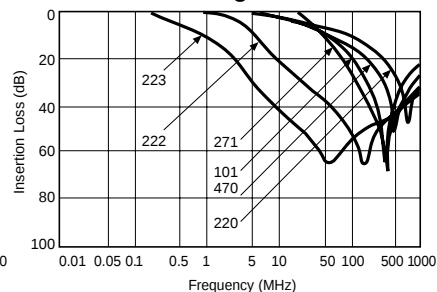
DSS310 Series Fig. 9 BL222/DL223
