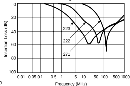
DST310 Series Fig. 5
