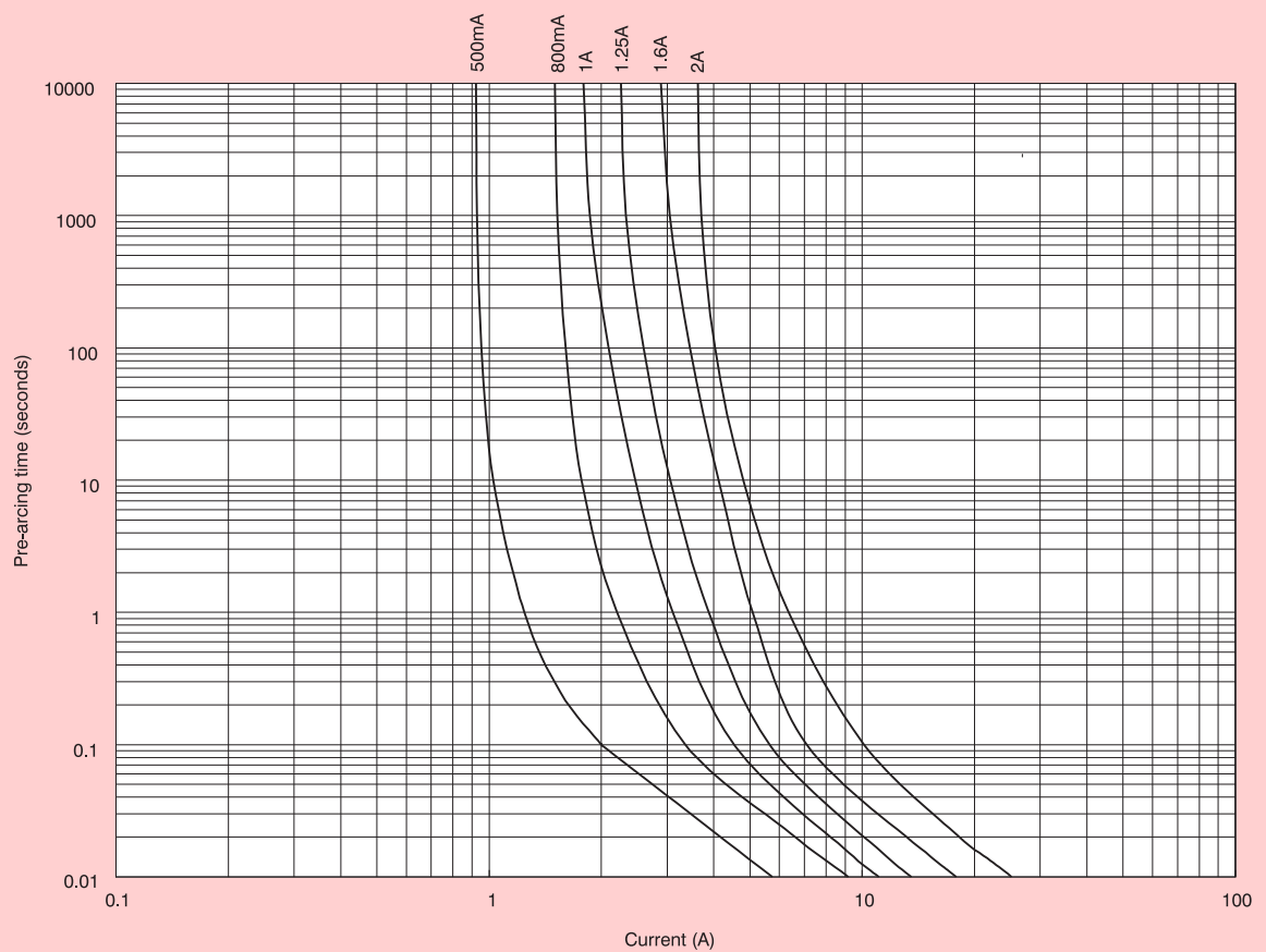
S505 Range: 500mA to 2A
