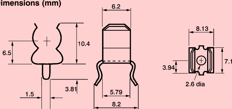
Dimensions (mm)
