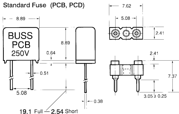
Standard Fuse (PCB, PCD)
