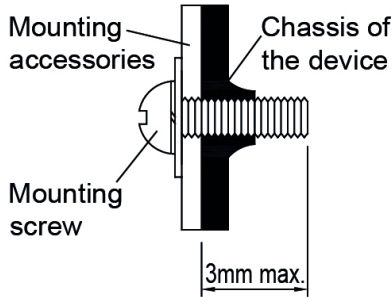
Fig. 5 Mounting Screw
