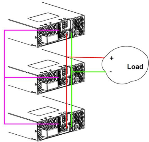
Parallel Connection with Remote Sense
