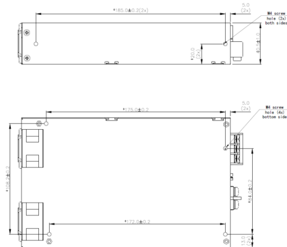
Fig. 4 Assembly Reference
