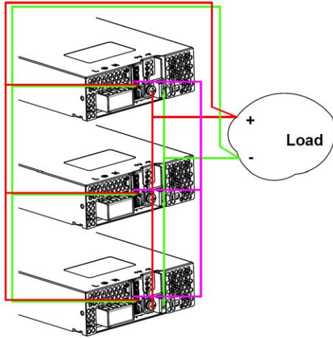
Parallel Connection without Remote Sense
