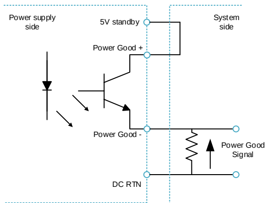
Fig. 10 Power Good Connection
