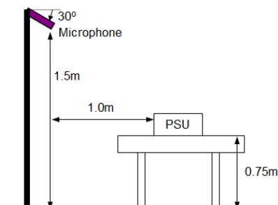
Fig 1. Acoustic Noise Testing Set Up
