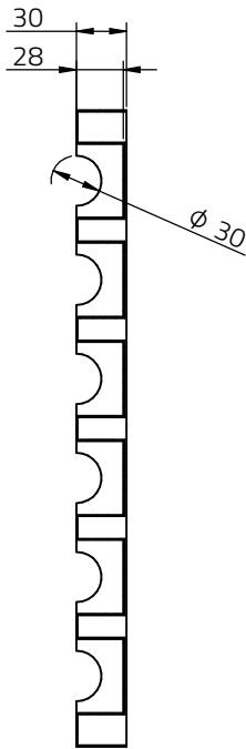
sectional drawing A-A
