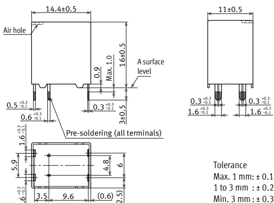
External dimensions
