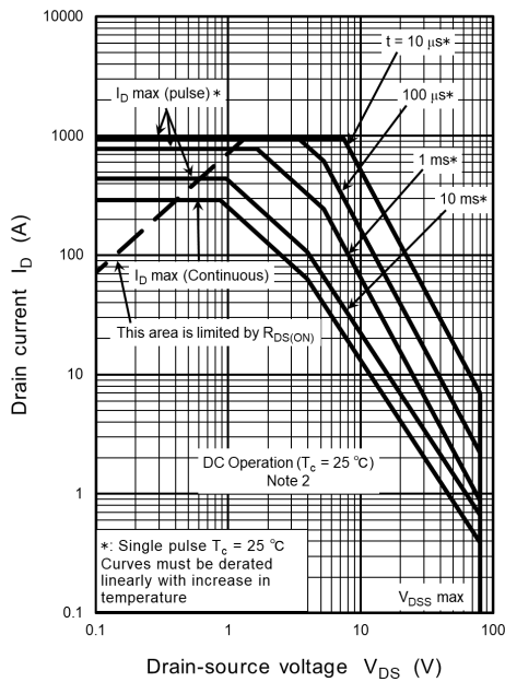
Fig. 8.16 Safe Operating Area (Guaranteed Maximum)
