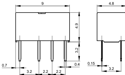
Outline Dimensions
