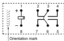
Single side stable
