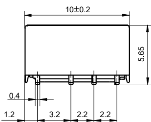
Short terminal SMT type
