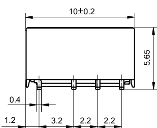
Standard SMT type
