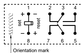
1 coil latching
