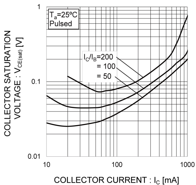
Fig.5 Collector-Emitter Saturation Voltage vs. Collector Current(II)
