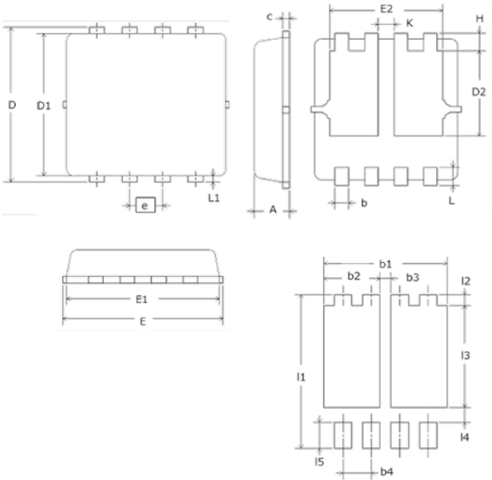
Referenced footprint dimensions
