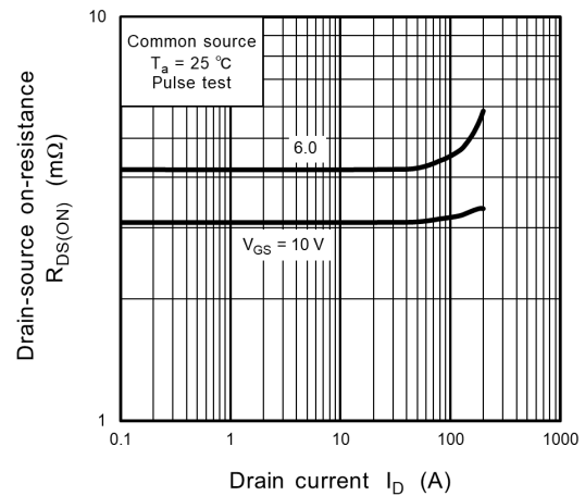
Fig. 8.8 R_{DS(ON)} - I_D
