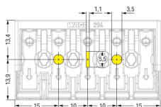
5-pole – with direct ground contact
